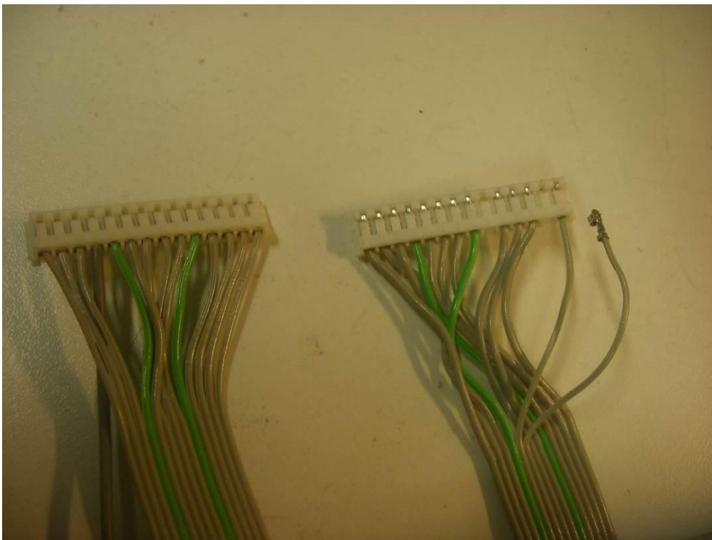
Left: cable with original wiring.
